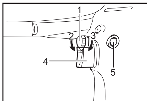
► 1. Speed control screw 2. Low 3. High 4. Switch trigger 5. Lock button
